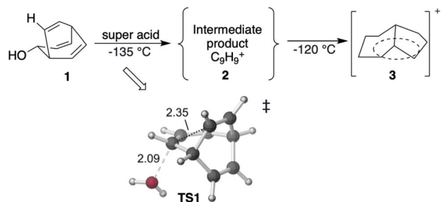
Scheme 1 Previous experiments on C_9H_9^+ cations. 50 The transition state TS1 is visualized using CYLVview 1.0 , 51 with key bond lengths labeled in Å. The C–O bond breaks first, and the C–C bond formation occurs subsequently in an asynchronous manner (see ESI† for details).
