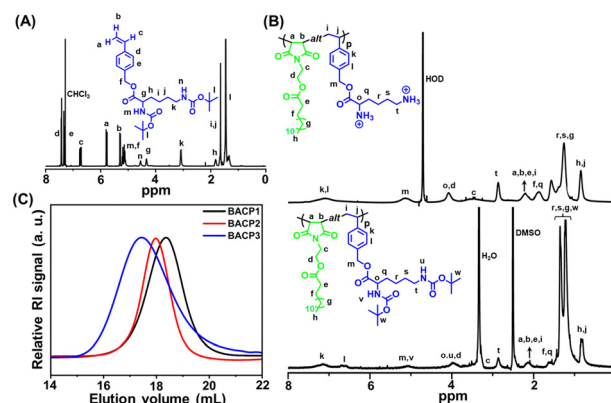
Fig. 1 (A) 1 H NMR spectrum of M2 . (B) 1 H NMR spectra of the protected polymer ( BACP3 ) in \text{DMSO}-d_6 and deprotected polymer ( ACPy ) in \text{D}_2\text{O} . (C) SEC RI traces of BACP1 – BACP3 in DMF.
