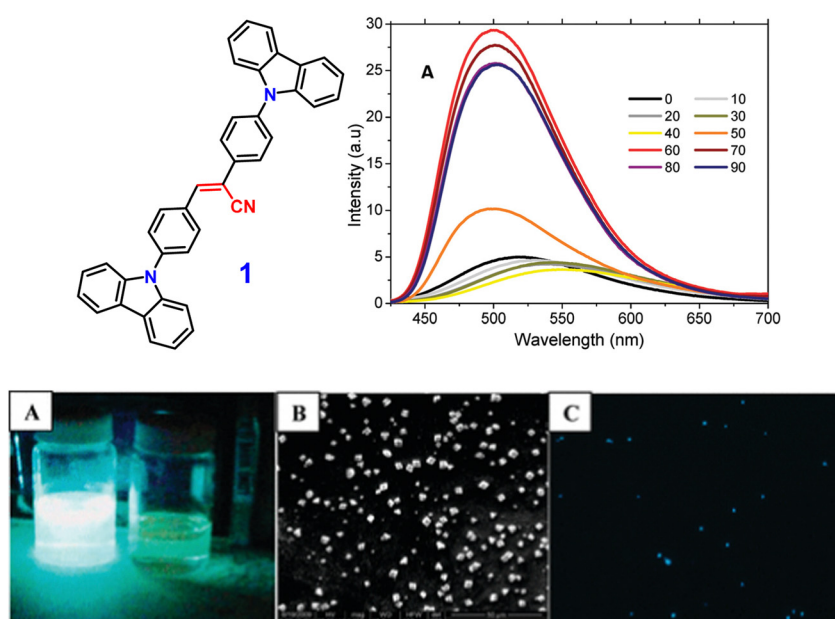
Fig. 2 Above: Structure of compound 1 (left), emission spectra of compound 1 in acetone–water mixtures; concentration = 10 \mu\text{M} , \lambda_{\text{exc}} = 360 nm (right). Below: (A) image of compound 1 taken in an acetone–water (40 : 60 v/v) mixture (left) and in pure acetone (right) under 365 nm UV light. (B) SEM image of compound 1 in an acetone–water (40 : 60 v/v) mixture. (C) Fluorescence microscopy image of microcrystals of compound 1 in an acetone–water (40 : 60 v/v) mixture. Reproduced with permission from ref. 70. Copyright 2011 the American Chemical Society.
