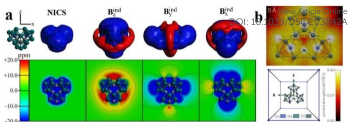
Fig. 8. (a) Isosurface and contour plot representation of the magnetic response properties for [\text{Co}_3@\text{Ge}_6\text{Sn}_{18}]^{5-} , denoting the NICS (isotropic/averaged) term, and from different orientations of the external field ( \mathbf{B}^{\text{ind}}_x , \mathbf{B}^{\text{ind}}_y , and \mathbf{B}^{\text{ind}}_z ). Isosurfaces set to \pm 8 ppm, blue: shielding; red: deshielding. (b) Current density of the [\text{Co}_3@\text{Ge}_6\text{Sn}_{18}]^{5-} cluster at the central plane located at 0 Å, containing the [\text{Co}_3\text{Ge}_3] ring. The calculations were performed at the PBE0/def2-TZVP level of theory, without including solvent effects. Reprinted with permission from 210 . Copyright 2025 American Chemical Society.
