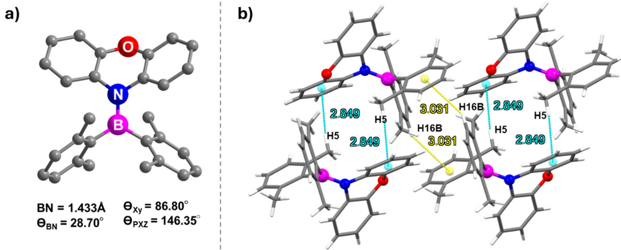
Fig. 2 (a) Molecular structure of BNO , and (b) supramolecular dimer chains of BNO . Cyan and yellow dashed lines represent the CH... \pi interactions. Atom colour code – carbon: grey, nitrogen: blue, oxygen: red, and hydrogen: off-white.
