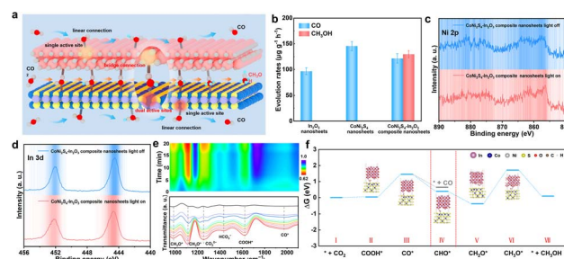
Fig. 6 (a) Schematic diagram of interlayer dual active site fixation intermediates promoting photoreduction of \text{CO}_2 to \text{CH}_3\text{OH} . (b) Rates of \text{CO}_2 photoreduction with different catalysts. Quasi in situ XPS spectra of (c) Ni 2p and (d) In 3d for the \text{CoNi}_2\text{S}_4\text{-In}_2\text{O}_3 composites of nanosheets. (e) In situ FTIR spectra and (f) free energy diagrams for the \text{CO}_2 photoreduction process on the \text{CoNi}_2\text{S}_4\text{-In}_2\text{O}_3 composite of the nanosheet slab. Reproduced with permission from ref. 54. Copyright 2024, American Chemical Society.
