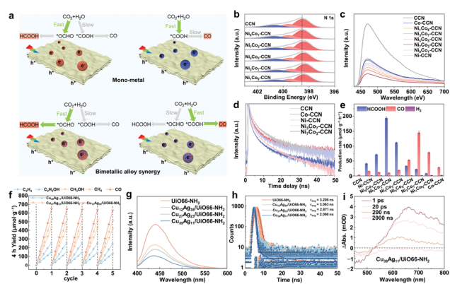
Fig. 5 (a) Schematic diagram of the reaction mechanism of photoreduction of \text{CO}_2 by the \text{Ni}_x\text{Co}_y\text{-CCN} catalyst. (b) XPS spectra of N 1s, (c) PL spectra and (d) time-resolved transient PL decay spectra for \text{Ni}_x\text{Co}_y\text{-CCN} . (e) Product evolution rates of \text{Ni}_x\text{Co}_y\text{-CCN} . Reproduced with permission from ref. 50. Copyright 2024, Wiley-VCH. (f) The cycling test over \text{CuAg}_{50-x}/\text{UiO66-NH}_2 . (g) PL spectra; (h) time-resolved transient PL decay spectra and (i) Fs-TA spectra of \text{CuAg}_{50-x}/\text{UiO66-NH}_2 . Reproduced with permission from ref. 51. Copyright 2024, Royal Society of Chemistry.
