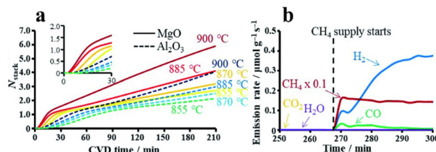
Fig. 2 Analysis of graphene growth reactions via CVD using CH 4 as a precursor on γ-Al 2 O 3 and MgO. (a) Plot of the number of graphene layers formed versus CVD reaction time. (b) Gas analysis during the CVD reaction on MgO. CH 4 was introduced to preheated MgO at 900 °C at the time labelled "CH 4 supply starts". Reprinted with permission. 33 Copyright Royal Society of Chemistry 2021.
