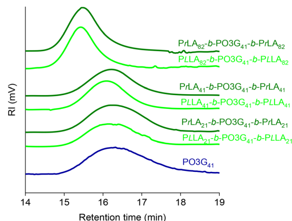
Fig. 2 SEC traces of the PO3G 41 macroinitiator and the PLA m - b -PO3G 41 - b -PLA m triblock copolymers.
