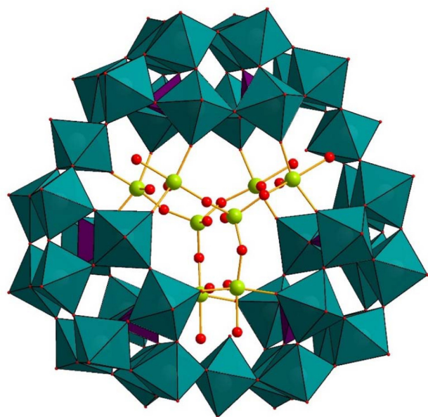
Fig. 11 Combined polyhedral/ball-and-stick representation of [\text{Rb}_3\text{C}\{\text{V}_4^{\text{IV}}\text{V}_2^{\text{IV}}\text{O}_{12}(\text{H}_2\text{O})_2\}_2\{\text{H}_6\text{P}_6\text{W}_{39}\text{O}_{147}(\text{H}_2\text{O})_3\}]^{15-} . Color code: \text{WO}_6 octahedra (green), \text{PO}_4 tetrahedra (pink), O (red), V (yellow). 93
