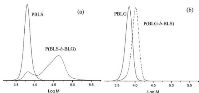
Fig. 4 SEC (HFIP) results of P(BLS- b -BLG) synthesis by sequential monomer addition. (a) Addition of BLG NCA to a PBLS macroinitiator (entry 1, Table 4) and (b) addition of BLS NCA to a PBLG macroinitiator (entry 4, Table 4).
