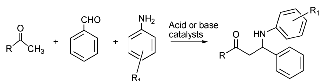
Scheme 8 Mannich reaction of aromatic aldehyde, ketones and amines.
