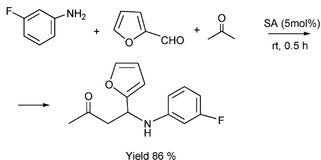
Scheme 10 Synthesis 4-(3-fluorophenylamino)-4-(furan-2-yl)butan-2-one.
