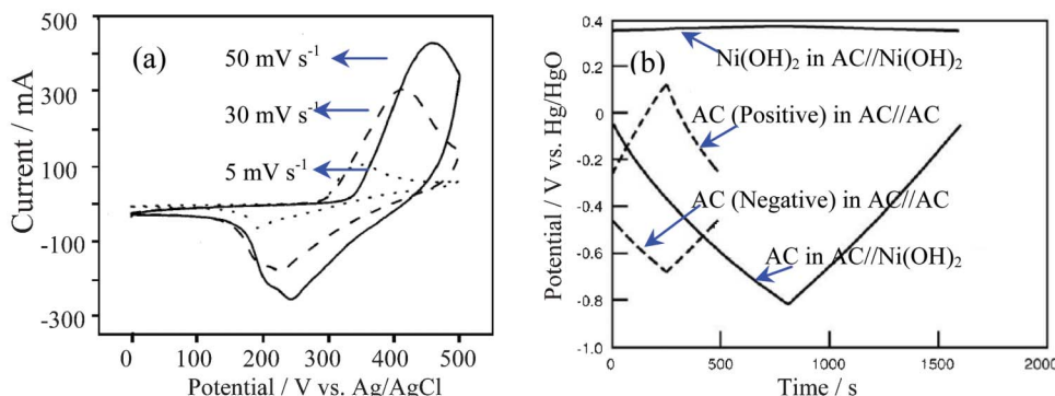
Fig. 15 (a) CV curve of \text{Ni}(\text{OH})_2 in alkaline solution and (b) charge/discharge curves of the positive and negative electrodes in the \text{AC}//\text{Ni}(\text{OH})_2 ASC and electric double layer capacitors of \text{AC}//\text{AC} at 1 \text{ mA cm}^{-2} in 10 \text{ mol l}^{-1} KOH aqueous solution (modified from ref. 87b and 90c).
