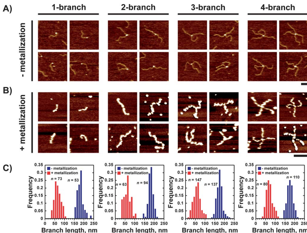
Fig. 2 AFM images of the four kinds of branched nanostructures before (A) and after (B) silver metallization prepared under the same conditions as in Fig. 1. All scale bars are 100 nm. The height scale is the same as that in Fig. 1B and C. (C) Branch length distributions before (blue) and after (red) metallization for each degree of branching. n shows the number of measured branches.
