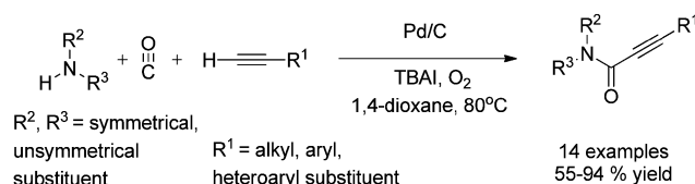
Scheme 42 Reagents and conditions: alk-1-yne (1 mmol), secondary amine (1.5 mmol), 10% Pd/C (8 mol%), \text{CO/O}_2 pressure (5/1 atm), TBAl (0.90 mmol), 1,4-dioxane (10 mL), temperature 80 °C, time 14 h.
