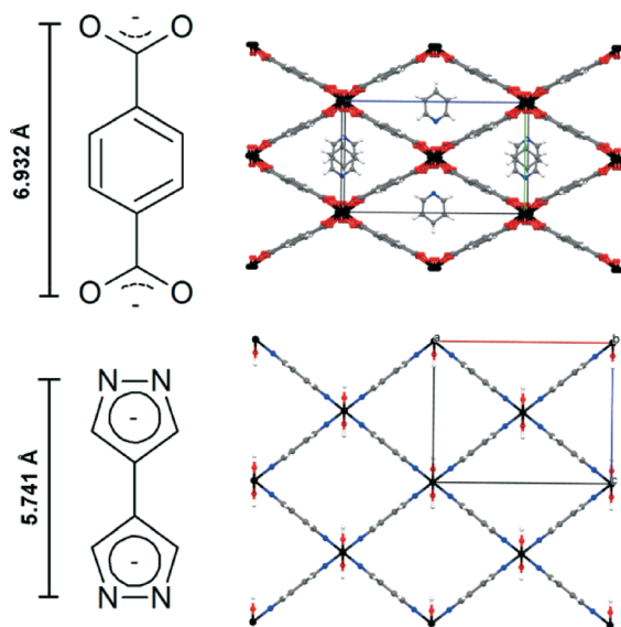
Fig. 1 Comparison of the terephthalate linker and the resulting MIL-53(Fe, as) structure and 4,4'-bipyrazolyl linker and the resulting Fe-CFA-6 structure. Distances between oxygen/nitrogen are obtained from crystallographic data (CIF files of MIL-53(Fe) and Fe-CFA-6).
