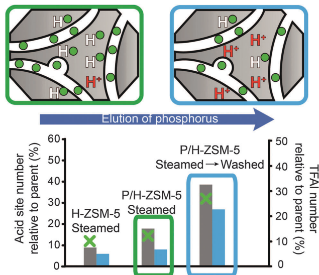
Fig. 11 Schematic representation of the recovery of the number of acid sites and TFAI species by washing after hydrothermal treatment. The acid site number is relative to the respective parent materials. Left axis: acid site number was determined using adsorption of pyridine. ■ = Lischke et al. 50 (steamed at 700 °C for 30 min. Washed using hot water) ■ = Blasco et al. 34 (steamed at 750 °C for 5 h. Washed using NH 4 F) right axis: TFAI number was determined using 27 Al MAS NMR. ■ = Lischke et al. (steamed at 700 °C for 30 min. Washed using hot water). 50
