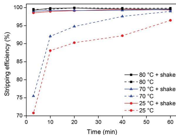
Fig. 9 Stripping kinetics and the influence of shaking (1500 rpm) are shown for 25\text{ }^{\circ}\text{C} , 70\text{ }^{\circ}\text{C} and 80\text{ }^{\circ}\text{C} with 1\text{ M} HCl. The cloud point temperature is 74\text{ }^{\circ}\text{C} and so at 80\text{ }^{\circ}\text{C} the system is one homogeneous phase which explains the efficient stripping without shaking. For 25\text{ }^{\circ}\text{C} and 70\text{ }^{\circ}\text{C} it consists of two phases, a water phase and an ionic liquid phase, making shaking essential for an efficient stripping process.
