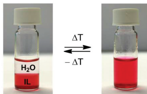
Fig. 8 Reversible formation of a homogeneous phase when increasing the temperature above the cloud point ( 55\text{ }^{\circ}\text{C} for a pure water/ionic liquid system in a 1:1 ratio). 44 A coloring agent (methyl red sodium salt) was dissolved in the transparent ionic liquid phase to help the visualization. The density of the [Hbet][Tf_2N] liquid is higher than that of water.
