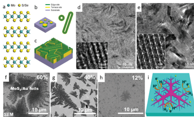
Fig. 3 (a) Layered crystal structure of molybdenum dichalcogenide. (b) Schematics of \text{MoS}_2 nanoparticle with platelet-like morphology distributed on a substrate (left), and nanotubes and fullerene-like nanotubes of \text{MoS}_2 and \text{MoSe}_2 (right). (c) Idealized structure of edge-terminated molybdenum dichalcogenide films with the layers aligned perpendicular to the substrate, maximally exposing the edges of the layers. TEM image of a \text{MoS}_2 film (d) and a \text{MoSe}_2 film (e) produced by rapid sulfurization/selenization, clearly showing exposed edges. High-resolution TEM image (inset) reveals individual layers consisting of three atomic planes in the sequence of S–Mo–S or Se–Mo–Se atomic planes (reproduced with permission from ref. 100. Copyright 2013 American Chemical Society). (f–i) HER activity of dendritic monolayer \text{MoS}_2 flakes transferred onto Au foils. (f–g) SEM images of monolayer \text{MoS}_2 flakes on Au foils with coverages of 60, 40 and 12% and domain sizes of \sim 10\ \mu\text{m} , \sim 5\ \mu\text{m} and \sim 800\ \text{nm} (in envelope edge length), respectively. (i) Schematic view illustrating the edges of fractal monolayer \text{MoS}_2 flakes as active catalytic sites for HER (reproduced with permission from ref. 101. Copyright 2014 American Chemical Society).
