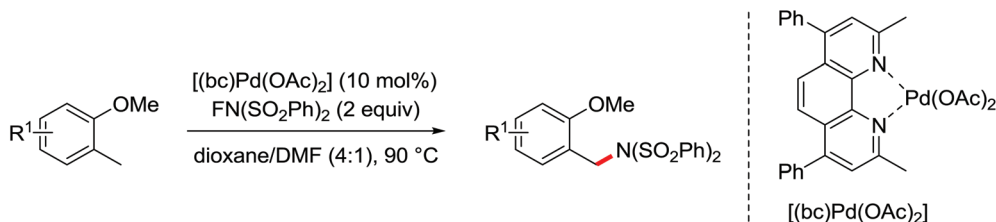
Scheme 363 Palladium-catalyzed C–H amidation of 2-methylphenyl ethers.
