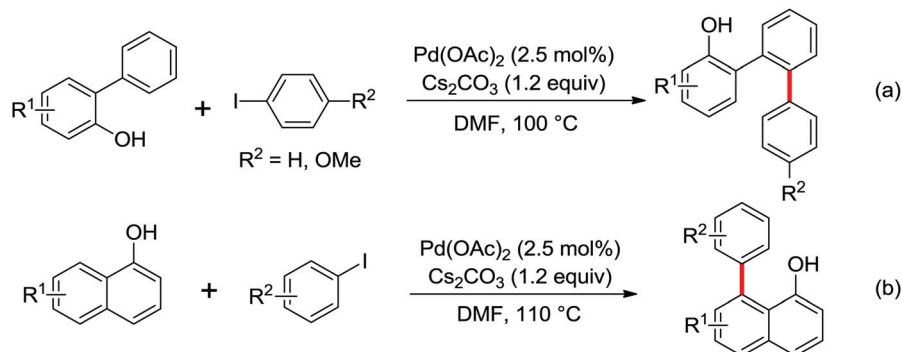
Scheme 330 Palladium catalyzed arylation of 2-phenylphenols and 1-naphthols.
