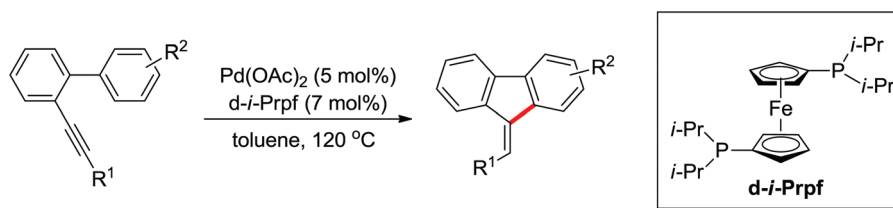
Scheme 394 Palladium-catalyzed intramolecular C–H activation of o -alkynylbiaryls.
