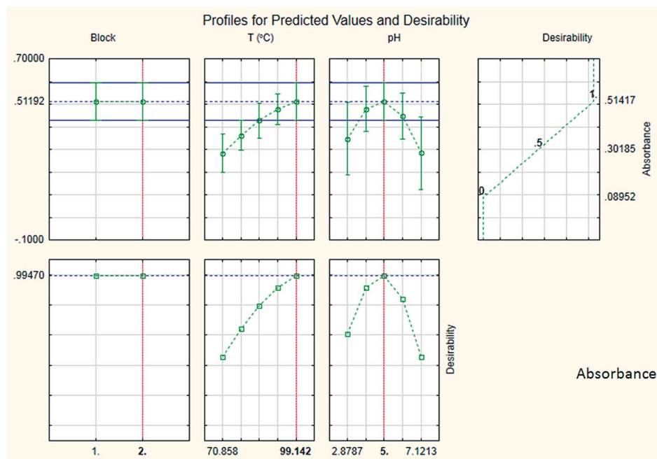
Fig. 7 Desirability function graph for CCD.
