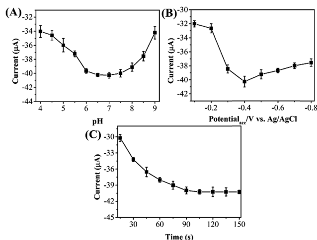
Fig. 4 Effect of the (A) pH of PBS, (B) accumulation potential and (C) accumulation time on the current response of 10 \mu\text{M} phoxim at RGO–Au/GCE.
