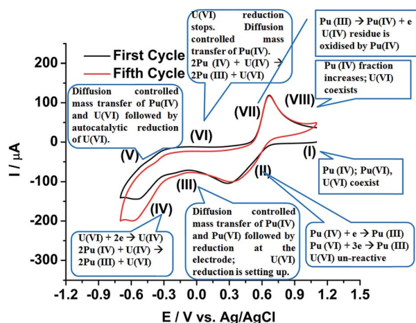
Fig. 9 Comprehensive representation of the autocatalytic reduction of U(vi) in the FBTR fuel sample solution containing both uranium and plutonium in 1 M \text{H}_2\text{SO}_4 .
