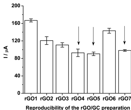
Fig. 11 ASWV peak currents of Pu(IV)/Pu(III) redox couple recorded on seven rGO/GCs in the final test solution ( i.e. ; sample + 3.047 \text{ mg g}^{-1} of standard Pu). The error bars represent the standard deviation for ten repetitive measurements. The arrows show the rGO/GCs selected for the ANOVA test.
