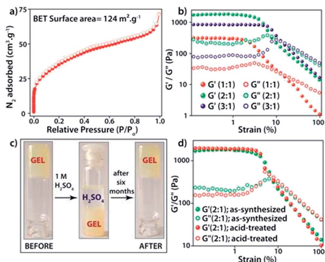
Fig. 3 (a) \text{N}_2 adsorption isotherm of FNPA (2 : 1) xerogel; (b) combined strain dependent studies of the FNPA metallogel (FN : PA (v/v) in DMF); (c) stability in 1 M \text{H}_2\text{SO}_4 for six months; (d) comparative strain sweep plot of as-synthesised and acid-treated FNPA metallogels (after six months).
