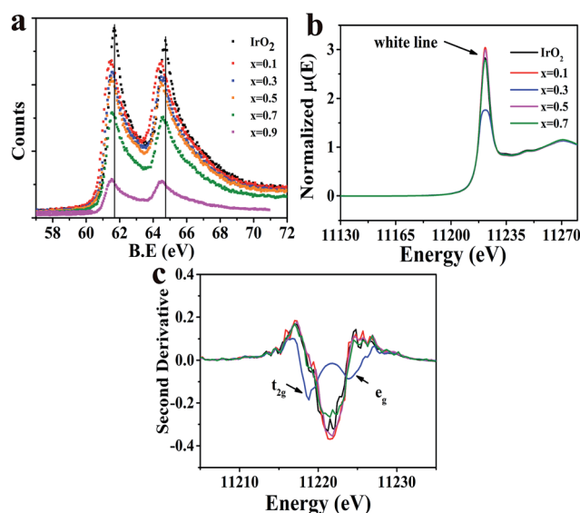
Fig. 5 (a) XPS spectra of Ir-4f in \text{Cu}_x\text{Ir}_{1-x}\text{O}_\delta compositions. The solid vertical lines correspond to the Ir-4f 7/2 and 4f 5/2 peak positions of \text{IrO}_2 . (b) Normalized Ir-L III edge XANES spectra for \text{Cu}_x\text{Ir}_{1-x}\text{O}_\delta compositions. (c) Second derivatives of Ir-L III edge XANES spectra for \text{Cu}_x\text{Ir}_{1-x}\text{O}_\delta compositions.
