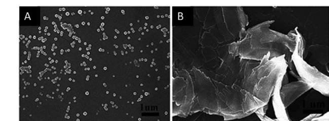
Fig. 34 Schematic representation of the anion- \pi induced self-assembly forming the vesicle as well as SEM images before (A) and after addition of 3 eq. of NaNO 3 (B). Reproduced with permission from John Wiley and Sons. 66
