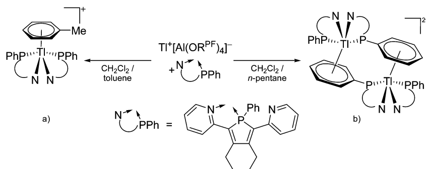
Fig. 28 Solvent effects on the formation of cationic thallium(i) complexes of NPPh. (a) If toluene is applied, the solvent-stabilized penta-coordinated [Tl(NPPh)_2(\eta^6-C_6H_5Me)]^+ complex forms. (b) If non-coordinating n -pentane is applied two [Tl(NPPh)]^+ cations aggregate via their phenyl substituents, forming the dinuclear and dicationic [Tl_2(NPPh)_4]^{2+} complex.
