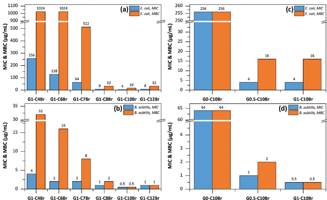
Fig. 5 MIC and MBC values of the QAS-functionalized dendron determined by serial dilution of dendron solutions (1–1024 μg mL -1 ) in a nutrient broth containing 10 6 CFU mL -1 of E. coli (a, c) or B. subtilis (b, d).
