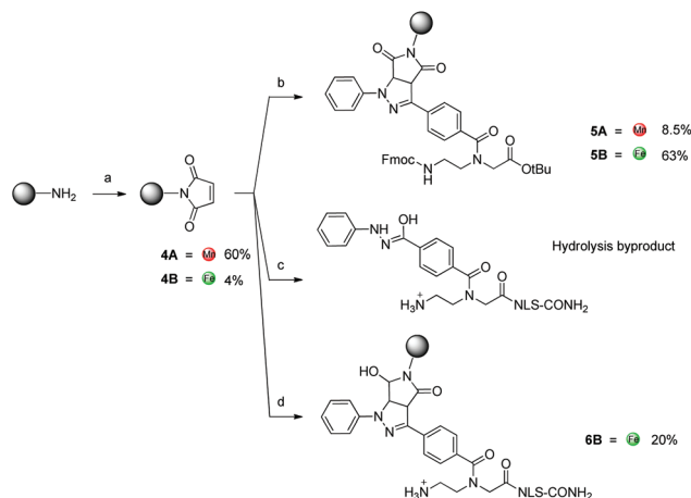
Fig. 5 Photoclick reaction. (a) Maleic anhydride, AcOH, 8 h, reflux. (b) 9 , ACN, 302 nm, 1 h, RT. (c) NLS-tetra, \text{H}_2\text{O} or ACN:PBS (5:1), 302 nm, 30 min, RT. (d) NLS-tetra, DMSO, 302 nm, 1 h, RT. All amine groups in the peptide sequence are present as TFA salts.
