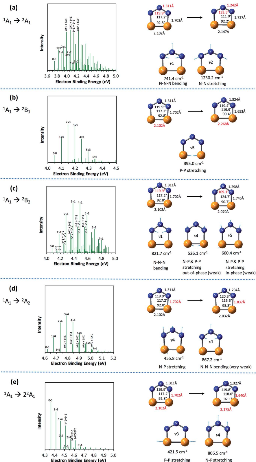
Fig. 4 Simulated vibrational progressions (stick spectra) at 20 K for the formation of the five low-lying states of P_2N_3^{\cdot-} from the ^1A_1 ground state of P_2N_3^- , using UB3LYP geometries, frequencies and FCFs, and UCCSD(T) energies. Geometry changes (the most significant changes are high-lighted in red) from the initial state of the anion to the target state of the radical and the active modes (with frequencies) for each of the five transitions are also shown. The assignments of the major peaks in the stick spectra are given.
