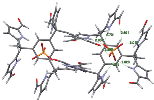
Fig. 5 Single crystal structure of the 2 : 2 complex [7b · \text{H}_2\text{PO}_4^- ] 2 . One TBA + counter cation per \text{H}_2\text{PO}_4^- and 1.5 molecules of \text{CHCl}_3 per 7b have been omitted for clarity.
