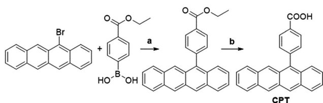
Scheme 1 Synthesis of transmitter tetracene derivative 4-(tetracen-5-yl)benzoic acid (CPT). Reagents and conditions: (a) \text{Cs}_2\text{CO}_3 , \text{Pd}(\text{dppf})\text{Cl}_2 \cdot \text{CH}_2\text{Cl}_2 , toluene : \text{H}_2\text{O} = 3 : 1, 60 °C, overnight. (b) 2 M KOH aqueous solution, THF : MeOH = 1 : 1, reflux, 3 h.
