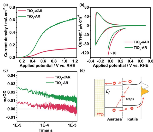
Fig. 4 (a) J-V curves of \text{TiO}_2 -dAR (red) and \text{TiO}_2 -AR (green). (b) Cyclic voltammograms curves of \text{TiO}_2 -dAR (red) and \text{TiO}_2 -AR (green) in \text{N}_2 purged 0.1 M \text{HClO}_4 . Scan rate: 50 \text{ mV s}^{-1} . (c) Transient absorption decay profiles of \text{TiO}_2 -dAR and \text{TiO}_2 -AR on the \mu\text{s} -ms timescale probed with a 550 nm excitation line at room temperature. A 75 W tungsten lamp and a Nd:YAG laser (355 nm) were used as the probe and the pump beam, respectively. (d) Schematic diagrams showing the possible charge transfer processes across the phase junction. The dotted arrows represent undesirable interface trapping/recombination processes.
