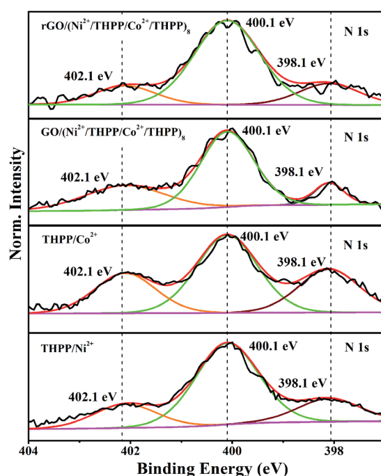
Fig. 2 High-resolution XPS spectra of N 1s of THPP/ \text{Ni}^{2+} , THPP/ \text{Co}^{2+} , \text{GO}/(\text{Ni}^{2+}/\text{THPP}/\text{Co}^{2+}/\text{THPP})_8 and \text{rGO}/(\text{Ni}^{2+}/\text{THPP}/\text{Co}^{2+}/\text{THPP})_8 .
