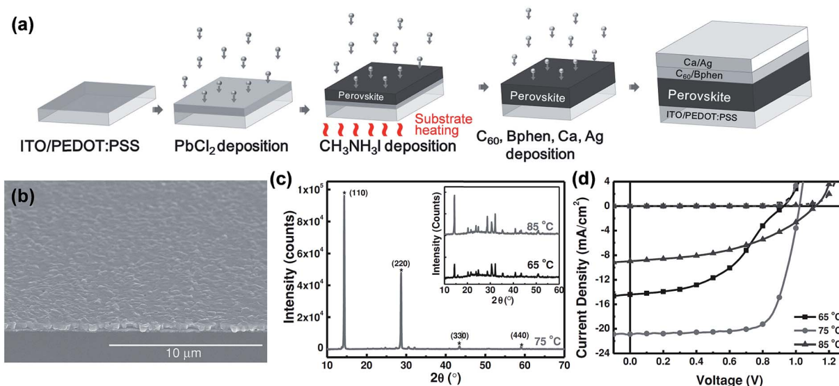
Fig. 8 (a) Schematic illustration for the fabrication of perovskite solar cell employing sequential layer-by-layer vacuum deposition. (b) Large area SEM image of the \text{CH}_3\text{NH}_3\text{PbI}_{3-x}\text{Cl}_x thin film fabricated with the substrate temperature held at 75 °C during \text{CH}_3\text{NH}_3 sublimation. (c and d) XRD and J - V characteristics of perovskite layers and solar cells with varying substrate temperatures (65 °C, 75 °C, 85 °C) during \text{CH}_3\text{NH}_3 sublimation. Reproduced with permission from ref. 88.
