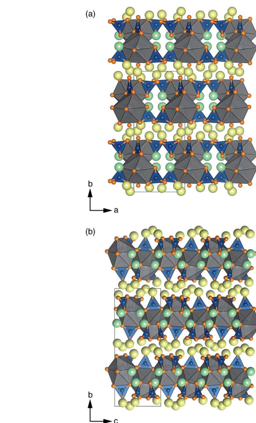
Fig. 1 Crystal structure of \text{Li}_6\text{Y}(\text{BO}_3)_3 . Illustration of the crystal structure of monoclinic \text{Li}_6\text{Y}(\text{BO}_3)_3 viewed along the (a) c - and (b) a -axis. B is shown in blue, Y in gray, O in orange, and Li in yellow or green. Edge-sharing \text{YO}_8 dodecahedra form chains that zig-zag along the c -axis. Trigonal bipyramidal chains of \text{LiO}_5 form along the c -direction and connect the chains of \text{YO}_8 along the a -direction.
