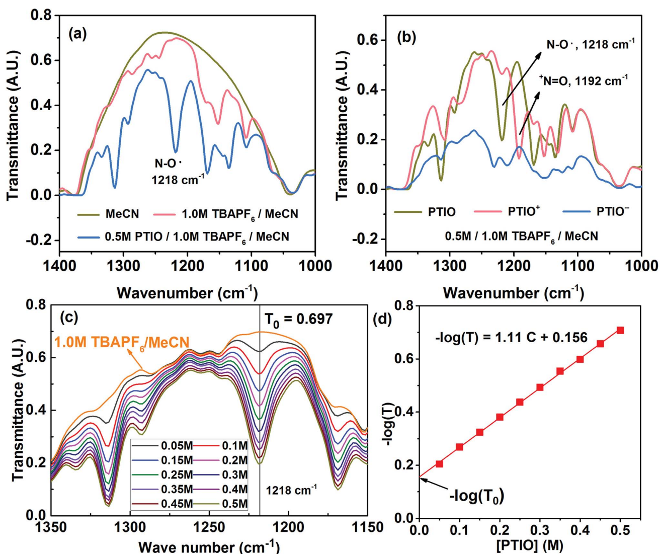
Fig. 4 FTIR of the PTIO species in the TBAPF 6 /MeCN electrolyte systems: (a) expanded spectral view for MeCN, 1.0 M TBAPF 6 /MeCN, and 0.5 M PTIO in 1.0 M TBAPF 6 /MeCN; (b) expanded spectral view of 0.5 M PTIO, PTIO + , and PTIO - ; (c) expanded spectral view of PTIO in 1.0 M TBAPF 6 with [PTIO] ranging from 0.05 M to 0.5 M; (d) derived linear -\log(T) vs. [PTIO] calibration curve based on the peak at 1218 \text{cm}^{-1} .
