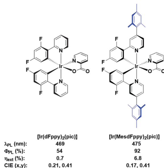
Fig. 2 FIrpPic and its mesityl functionalised analogue. The mesityl functionality confers improved properties in virtually all important metrics, including solution state \Phi_{\text{PL}} , as well as \eta_{\text{ext}} values and CIE coordinates for comparable solution processed device architectures. This comes only at the expense of a small red-shift in solution state \lambda_{\text{max}} .
