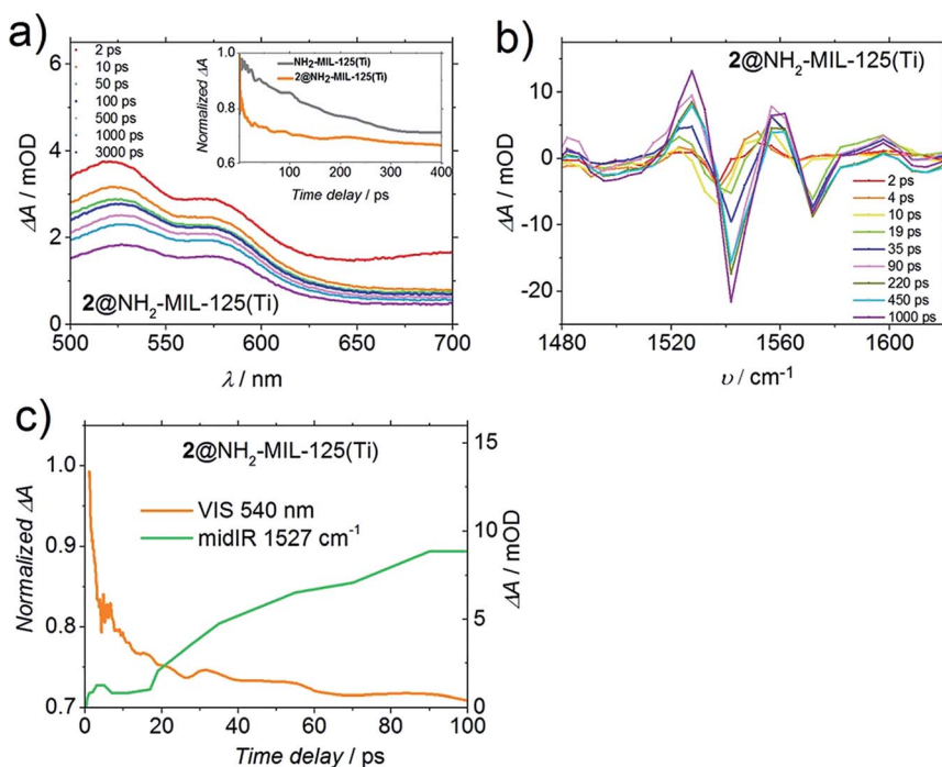
Fig. 6 (a) Differential transient spectra of 2@ \text{NH}_2\text{-MIL-125}(\text{Ti}) in DMF upon excitation at 400 nm, inset: comparison of the time traces of \text{NH}_2\text{-MIL-125}(\text{Ti}) and 2 occluded in \text{NH}_2\text{-MIL-125}(\text{Ti}) at 540 nm in DMF, (b) differential transient absorption mid-IR spectra for 2@ \text{NH}_2\text{-MIL-125}(\text{Ti}) in DMF upon excitation at 400 nm, and (c) representative time traces of 2@ \text{NH}_2\text{-MIL-125}(\text{Ti}) upon excitation at 400 nm in DMF recorded at 1527 \text{ cm}^{-1} (green). The orange line (corresponding to the left axis) represents the time traces at 540 nm in DMF (same as in (a), inset orange line).
