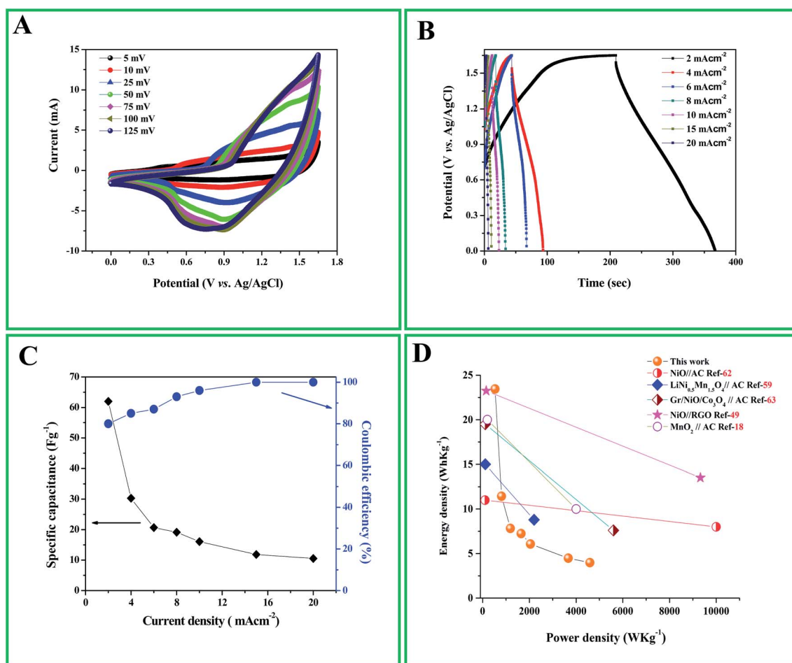
Fig. 6 (A) CV curves of ASC fabricated using Ni/Ni(OH) 2 //AC at various scan rates; (B) galvanostatic charge/discharge (GCD) curves of ASC at various current densities. (C) Specific capacitance and coulombic efficiency as function of current density for ASC; (D) Ragone plot comparison with previous reports.
