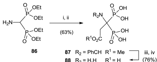
Scheme 22 Reagents and conditions: (i) m\text{-ClC}_6\text{H}_4\text{CHO} , \text{MgSO}_4 , \text{CH}_2\text{Cl}_2 . (ii) \text{BrCH}_2\text{CO}_2\text{Me} , \text{Bu}_4\text{NBr} , \text{K}_2\text{CO}_3 , MeCN. (iii) 1 N HCl, MeCN; then NaOH. (iv) 6 N HCl.
