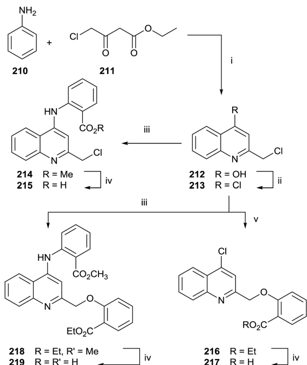
Scheme 37 Reagents and conditions: (i) PPA, 130^\circ\text{C} , 1 h. (ii) \text{POCl}_3 , 100^\circ\text{C} , 3 h. (iii) Methyl 2-aminobenzoate, \text{C}_2\text{H}_5\text{OH} , conc. \text{HCl} , 5 h. (iv) \text{THF}/\text{MeOH} , \text{LiOH} , 3 h. (v) Ethyl-2-hydroxybenzoate, \text{K}_2\text{CO}_3 , \text{CH}_3\text{CN} , 90^\circ\text{C} , 5 h.
