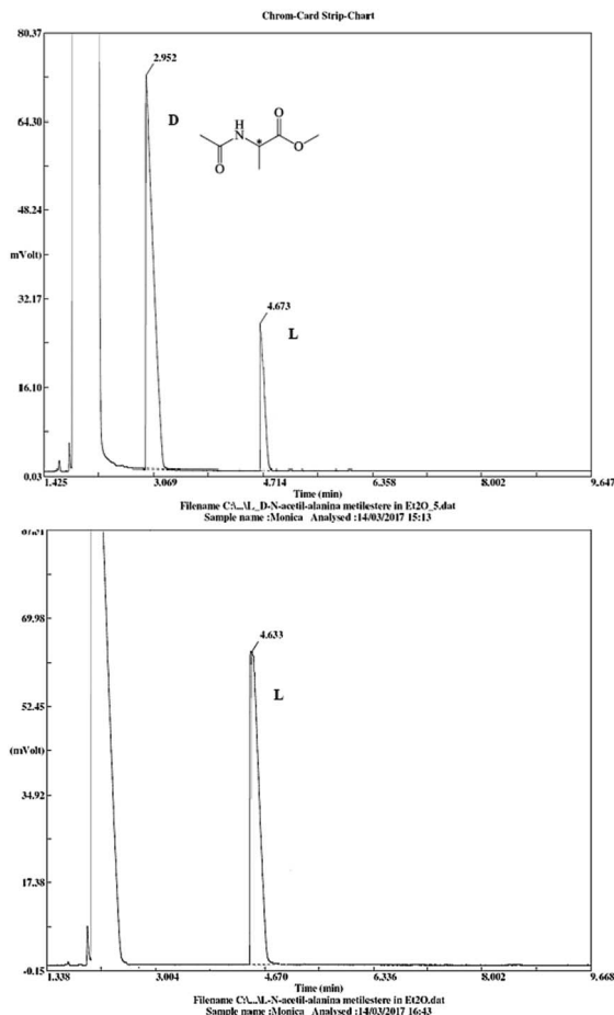
Fig. 1 Chiral GC data for Ac-DL-Ala-OMe and Ac-L-Ala-OMe (25 m × 0.25 mm, diethyl tert -butyldimethylsilyl-β-cyclodextrin chiral capillary column).
