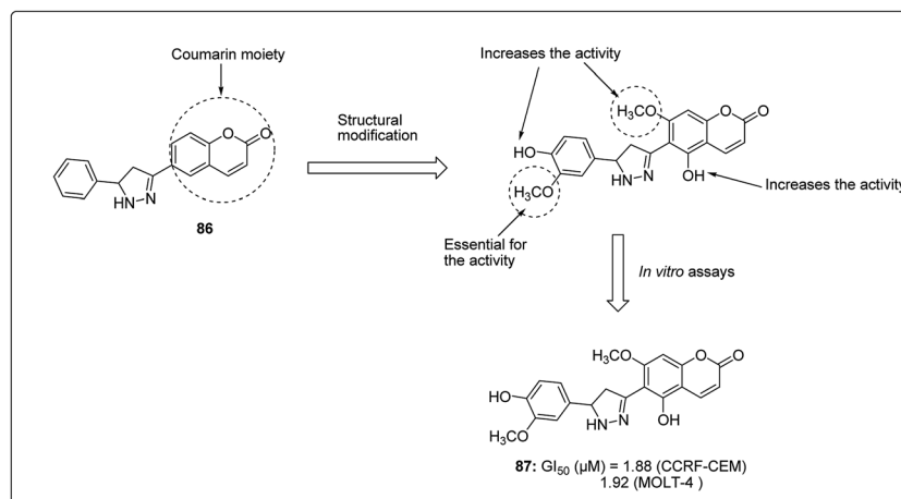
Fig. 19 Structure of most active 6-pyrazolinylcoumarin analogue as anticancer agent.
