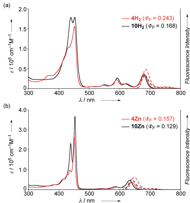
Fig. 1 UV/Vis absorption and emission spectra of (a) 4H 2 and 10H 2 , and (b) 4Zn and 10Zn in CH 2 Cl 2 . ε = extinction coefficient.
