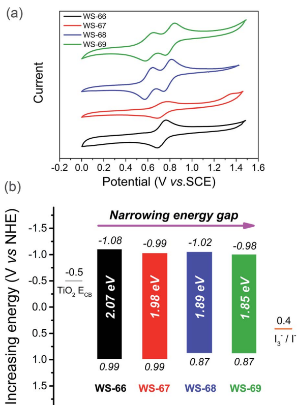
Fig. 3 Cyclic voltammograms of dyes WS-66 , WS-67 , WS-68 and WS-69 measured in CH 2 Cl 2 (a), LUMO (above the coloured bar) and HOMO (under the coloured bar) values, and energy band gaps of dyes WS-66 , WS-67 , WS-68 and WS-69 (b).
