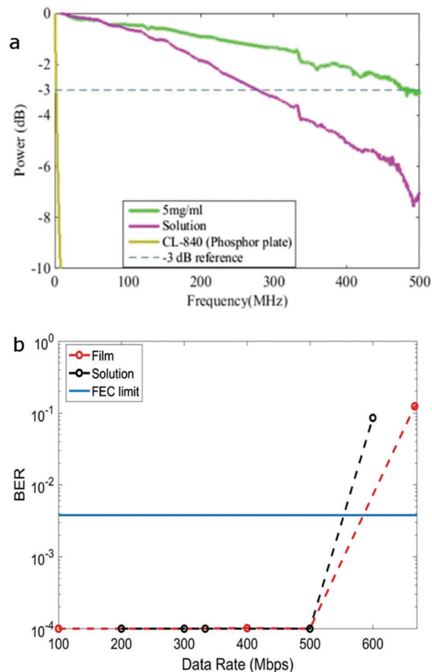
Fig. 2 Top: Plot of electrical power vs. frequency – BBEHBO–PPV films and solution. The dotted line shows the reference –3 dB bandwidth point. The frequency response of commercial phosphor plate (CL-840) is also shown for comparison. Bottom: Bit Error Rate (BER) vs. data rate using PAM-2 of BBEHBO–PPV films and solution.
