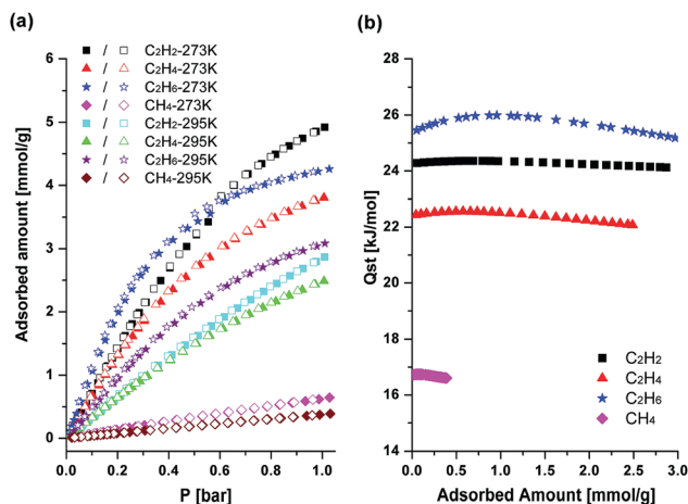
Fig. 3 (a) The adsorption isotherms of HOF-BTB for C 2 H 2 , C 2 H 4 , C 2 H 6 and CH 4 at 273 K and 295 K, respectively, and (b) loading dependent isosteric heat of adsorption. The Q_{st} values were calculated based on adsorption isotherms at 273 K and 295 K by using the Virial method.
