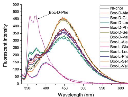
Fig. 2 Fluorescence changes of NI-cholesterol 1 (10 \mu M ) in CH_3CN –DMSO (95:5, v/v) with D and L isomers of Ala, Glu, Leu, Phe, Ser and Val (500 \mu M ). ( \lambda_{ex} = 325 nm, slit 3 \times 5).
