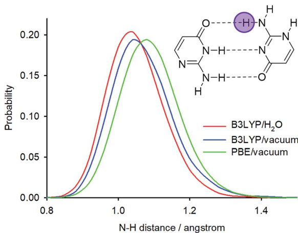
Fig. 8 \text{N2}'\text{-H2}^{\text{b}} distance probability distributions obtained from PIMD simulations at different computational levels.
