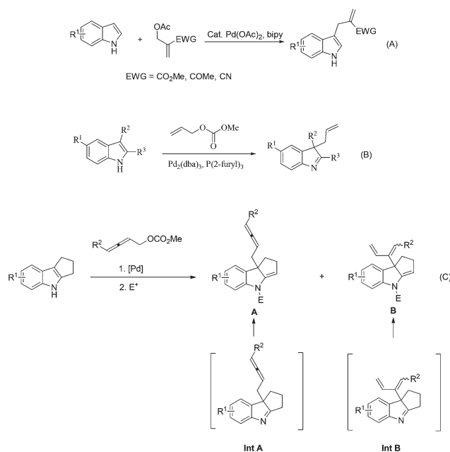
Scheme 1 (A) Palladium-catalyzed functionalization of electron-deficient alkenes with indoles. (B) Dearomatization of indoles derivatives with allylic carbonate. (C) Dearomatization of hydrocycloalk[b]indoles with 2,3-allenyl carbonates.
