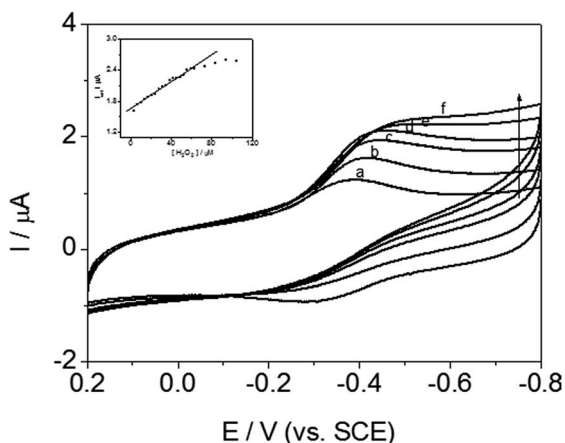
Fig. 11 Cyclic voltammograms of DM-EB/Hb/GCE with (a) 0\text{ }\mu\text{mol L}^{-1} , (b) 3.5\text{ }\mu\text{mol L}^{-1} , (c) 24.5\text{ }\mu\text{mol L}^{-1} , (d) 31.5\text{ }\mu\text{mol L}^{-1} , (e) 63.0\text{ }\mu\text{mol L}^{-1} and (f) 84.0\text{ }\mu\text{mol L}^{-1} \text{H}_2\text{O}_2 in PBS (pH 7.0), and plots of the electrocatalytic current ( I_{\text{cat}} ) vs. \text{H}_2\text{O}_2 concentration on DM-EB/Hb/GCE (inset). Scanning rate, 200\text{ mV s}^{-1} .
